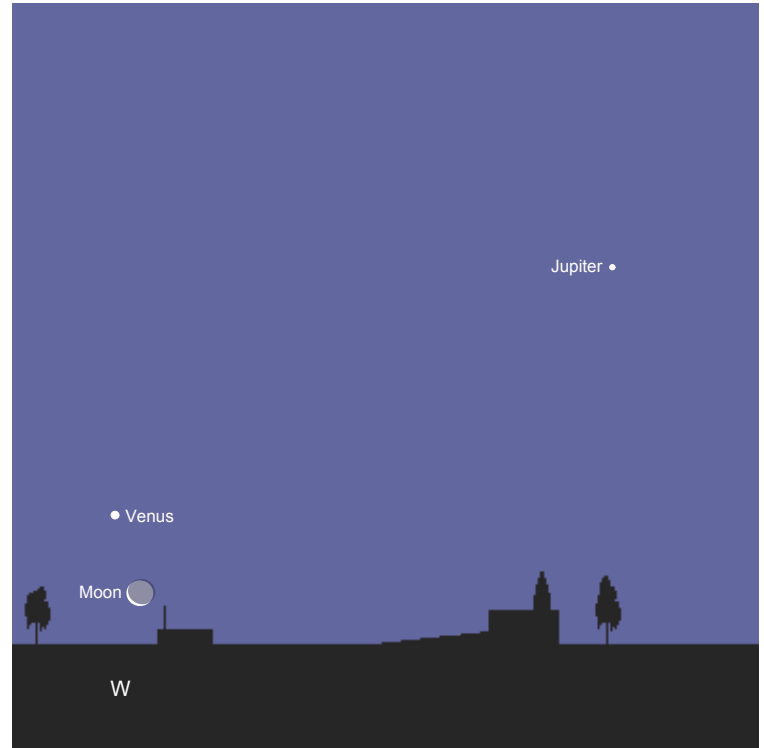
Southern Hemisphere view as seen from Sydney, Australia (34S) - 1 hour after sunset
